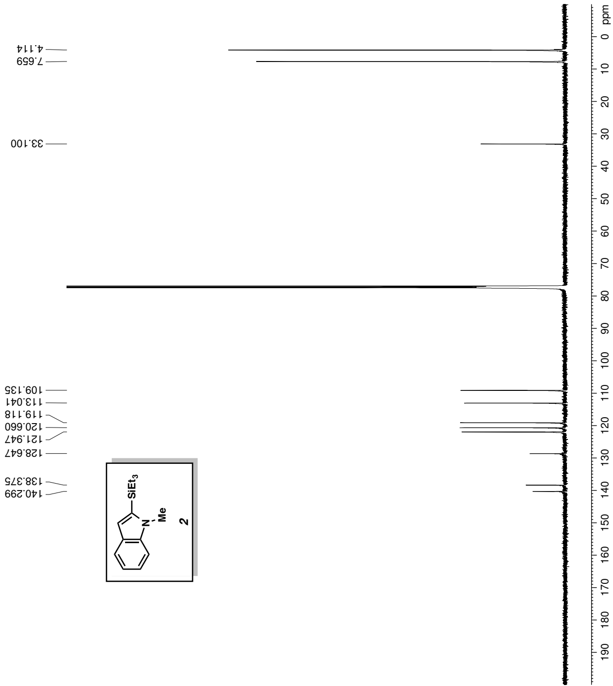
13 C NMR for compound (2)
